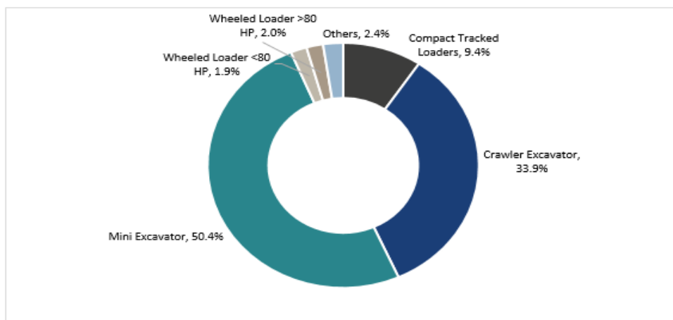
Japan Construction Machinery - Unit Production by Category (%), (212,000 units in 2020)
